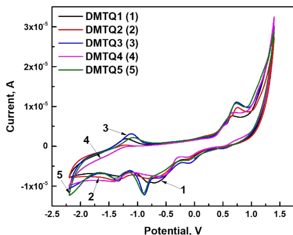
Figure 4. Cyclic voltammograms of DMTQ1-DMTQ5 recorded in DMF containing 0.1 M TBAPF 6 at a scan rate of 50 mV/s using a Pt working electrode, Pt counter electrode, and Ag/AgCl reference electrode.
