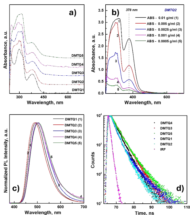
Figure 1. Photophysical properties of DMTQ derivatives in solution. (a) UV-Vis absorption spectra of DMTQ1-DMTQ5 (measured in \text{CHCl}_3 , c = 1 \times 10^{-5} M); (b) Concentration-dependent absorption spectra of DMTQ2 in \text{CHCl}_3 (0.01–0.0005 g/ml); (c) Normalized photoluminescence (PL) spectra of DMTQ1-DMTQ5 in \text{CHCl}_3 ( \lambda_{\text{exc}} = 375 nm, c = 0.005 g/ml); (d) Time-resolved PL decay profiles of DMTQ1-DMTQ5 in \text{CHCl}_3 ( \lambda_{\text{exc}} = 375 nm, \lambda_{\text{em}} = 505 nm).
