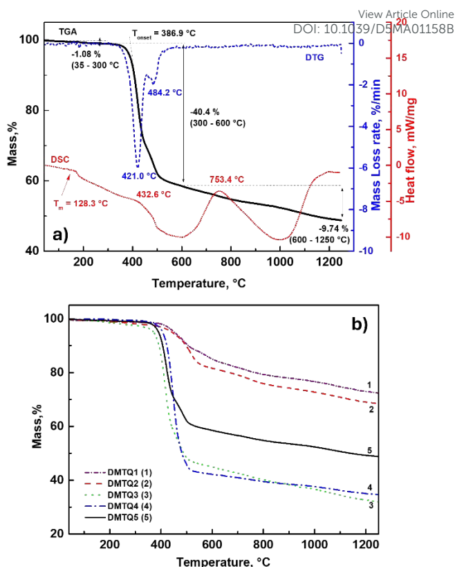
Figure 3. (a) Combined thermogravimetric (TGA, black solid), derivative thermogravimetric (DTG, blue dashed), and differential scanning calorimetry (DSC, red dotted) profiles of sample DMTQ5 , measured simultaneously under nitrogen atmosphere ( 50 \text{ ml}\cdot\text{min}^{-1} ) at a heating rate of 10 \text{ }^\circ\text{C}\cdot\text{min}^{-1} . The graph also indicates the evaluated parameters, including mass changes, T_{\text{onset}} , melting temperature, and the peak maxima of DTG and DSC signals associated with the observed decomposition. (b) Comparison of thermogravimetric (TGA) curves for all synthesized compounds DMTQ1-DMTQ5 measured under nitrogen atmosphere.
