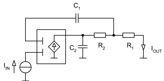
Fig.18 Final circuit diagram.
