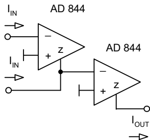
Fig.16 Solution with two transimpedance amplifiers
