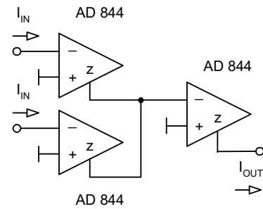
Fig.17 Solution with three transimpedance amplifiers
