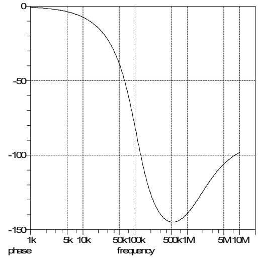
Fig.12 Proposed circuit phase response
