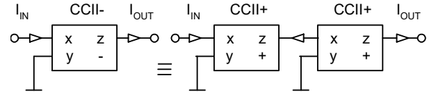
Fig.7 Realization CCII- from a pair of CCII+
