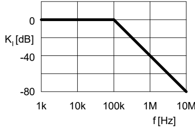
Fig.9 Proposed circuit Bode magnitude plot
