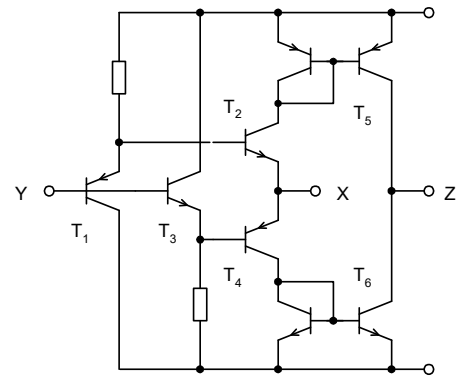
Fig.3 Simplified current conveyor schematic diagram
