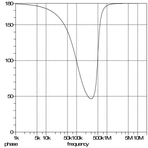
Fig.11 Original circuit phase response
