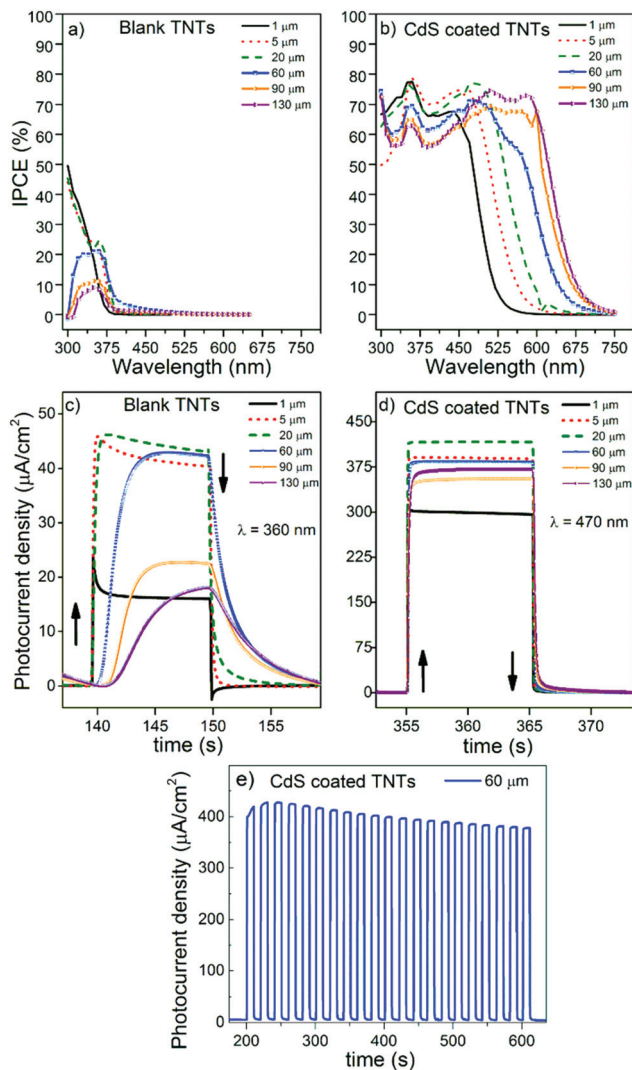
Fig. 5 (a and b) Incident photon-to-current efficiency and (c and d) transient photocurrent at 360 nm and at 470 nm, respectively, recorded for blank and CdS/TiO 2 nanotube layers of different thicknesses. Arrows indicate light ON (↑) and light OFF (↓). (e) Cycling performance of photocurrent transients, measured at 470 nm for 60 μm thick CdS coated TiO 2 nanotube layers (21 cycles).
