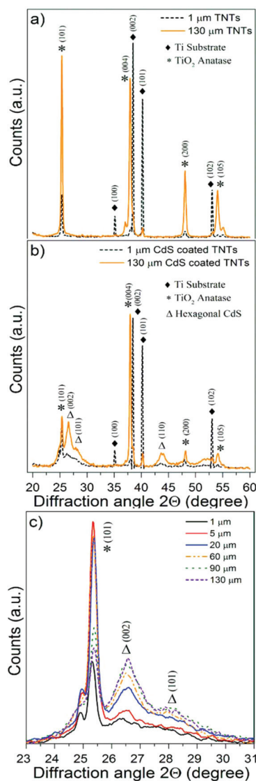
Fig. 4 XRD pattern of the (a) blank and (b) CdS coated TiO 2 nanotube layers 1 and 130 μm thick. (c) Details of the anatase peak corresponding to the plane (101) and CdS peaks associated to planes (002) and (101) obtained from all the CdS/TiO 2 nanotube layers.
