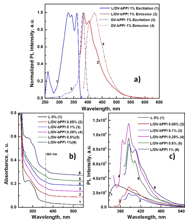
Fig. 4 Excitation and emission spectra of the L/DV-bPPI 1% polymer film (solid lines) in comparison with excitation and emission spectra of the PPI derivative (dashed lines) (a); absorbance spectra of L/DV-bPPI films with different DV-bPPI content (b); PL spectra of L/DV-bPPI films with different DV-bPPI content (c)
