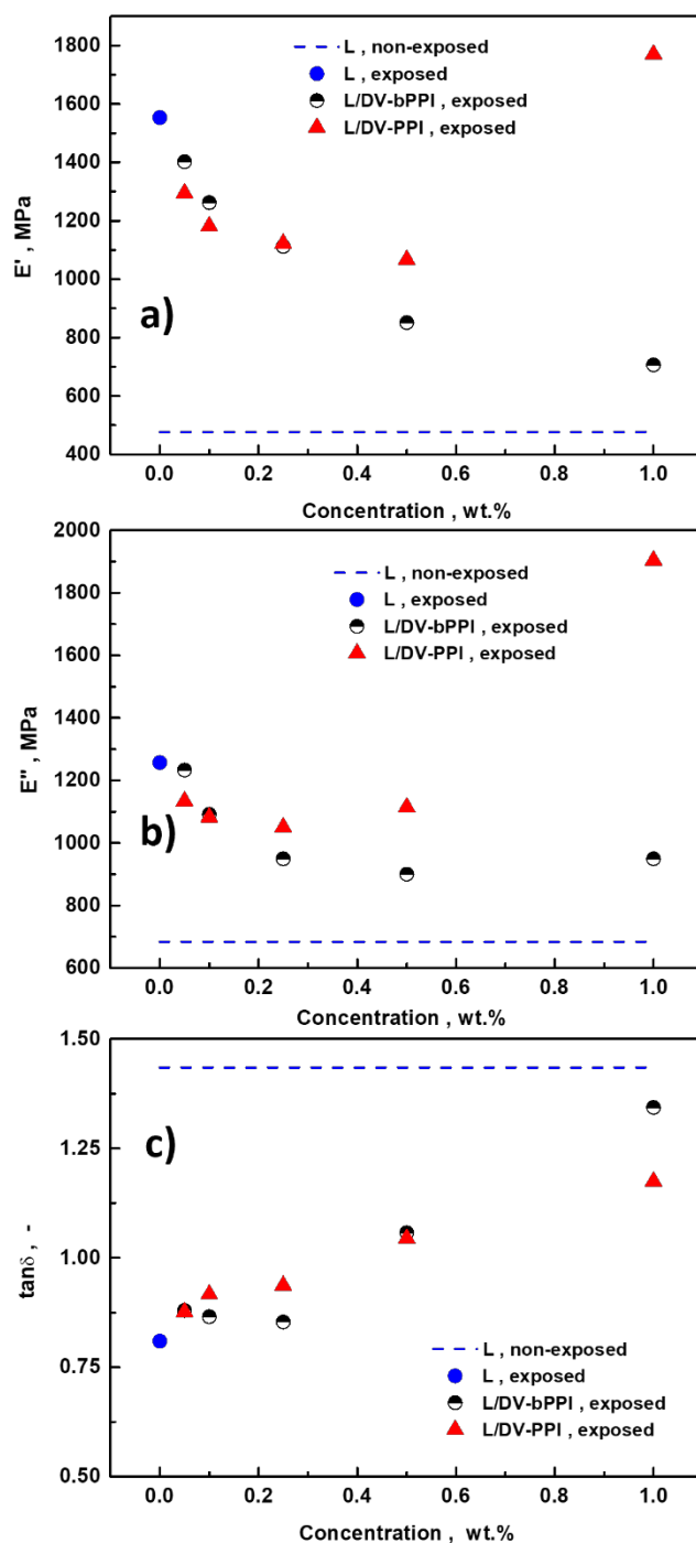
Fig. 16 Mechanical properties evaluated using DMA for the latex films exposed to UV irradiation, in contrast to the non-exposed reference latex film L 0%.
