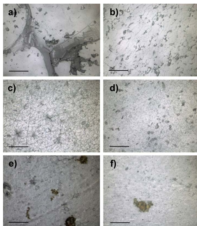
Fig. 11 Micrographs for the latex films containing DV-bPPI derivative at different concentrations: L/DV-bPPI 0.05% exposed to UV irradiation (a), L/DV-bPPI 0.1% exposed to UV irradiation (b), L/DV-bPPI 0.25% exposed to UV irradiation (c), L/DV-bPPI 0.5% (d), L/DV-bPPI 1% exposed to UV irradiation (e), L/DV-bPPI 1% non-exposed (f). The scale bars indicate 200 \mu\text{m}
