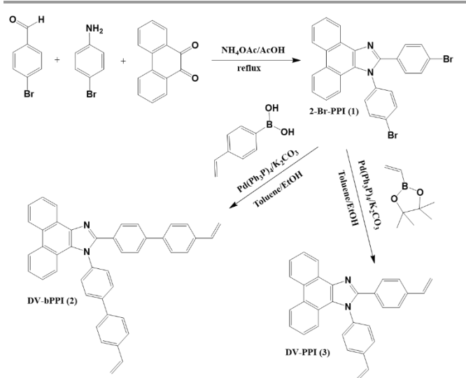
Fig. 1 Synthetic route of the target UVAs
