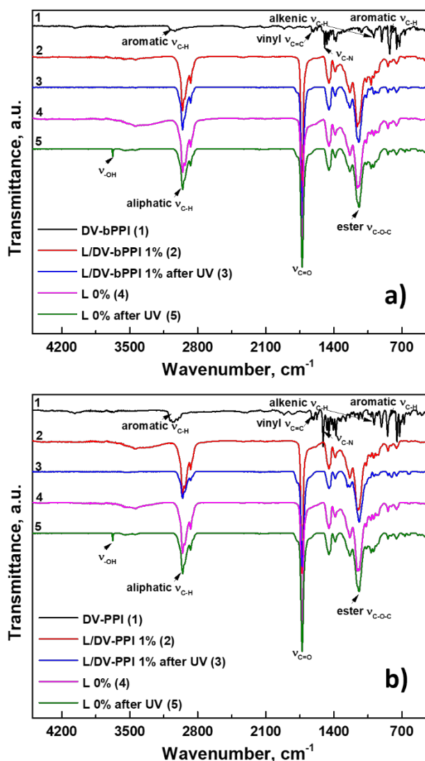
Fig. 14 FTIR spectra of monomers (UVAs), unexposed and UV-exposed latexes
