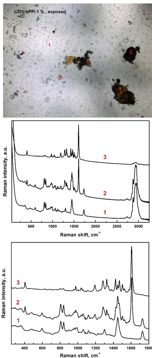
Fig. 13 Representative micrograph obtained for L/DV-bPPI 1% latex film exposed to UV irradiation; the numbers 1 – 3 denote various morphological features. Features denoted with no. 1 include all types of defects commonly observed for all non-exposed and exposed L/DV films. The Raman spectra (depicted in full scale as well as zoomed-in on the region of main bands) then correspond in their denotation to the archetypal features depicted in the micrograph
