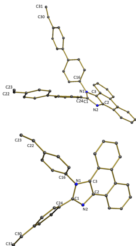
Fig. 2 Molecular structures of DV-bPPI and DV-PPI
