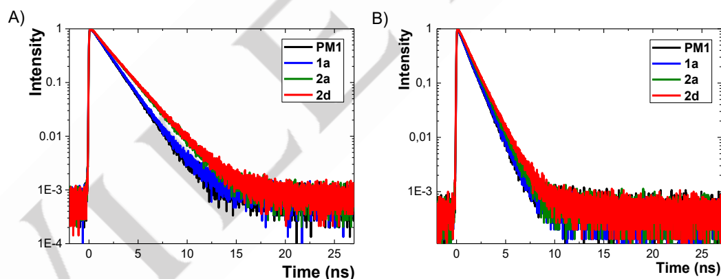
Figure 4. Fluorescence decays in the ns timescale for fluorophores PM1 (4-H), 1a (4-F), 2a (4- \text{CF}_3 ), and 2d (4- \text{SF}_5 ) measured in A) THF and B) toluene ( c \approx 5 \times 10^{-6} \text{ M} ).
