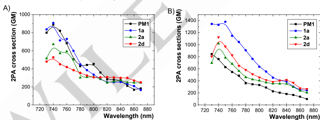
Figure 6. Two-photon absorption spectra for fluorophores PM1 (4-H), 1a (4-F), 2a (4-CF 3 ), and 2d (4-SF 5 ) measured in A) THF and B) toluene.
