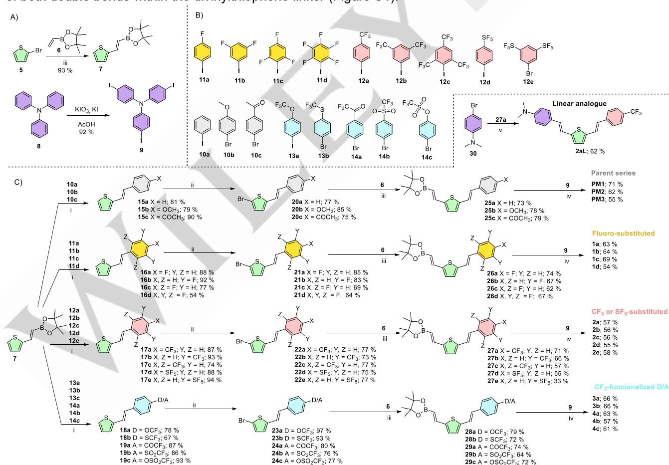
Scheme 1. Synthetic pathways towards tripodal fluorophores 1–4 . A) Synthesis of the key intermediates 7 and 9 . B) Structures of the starting bromo or iodobenzenes bearing fluoro acceptors. C) Straightforward four-step reaction pathway towards all target fluorophores PM1–3 and 1–4 : i) 7 (1.1 eq), [PdCl 2 (PPh 3 ) 2 ] (0.02 eq), K 2 CO 3 (1.5 eq), THF/H 2 O 4:1, 60 °C, 18 h; ii) NBS (1.05 eq), CHCl 3 /AcOH 2:1, 80 °C, 18 h; iii) vinylboronic acid pinacol ester 6 (1.5 eq), [Pd 2 (dba) 3 ] (0.01 eq), P( t Bu) 3 (0.05 eq), DIPEA (2 eq), toluene, 95 °C, 18 h; iv) corresponding boronic
