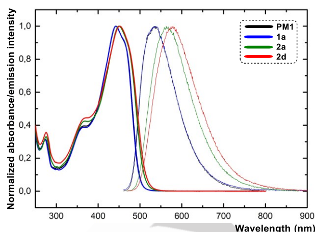
Figure 3. Normalized UV-Vis absorption (bold line) and emission spectra (thin line) of fluorophores PM1 (4-H), 1a (4-F), 2a (4- \text{CF}_3 ), and 2d (4- \text{SF}_5 ) measured in THF ( c \approx 5 \times 10^{-6} \text{ M} ).
