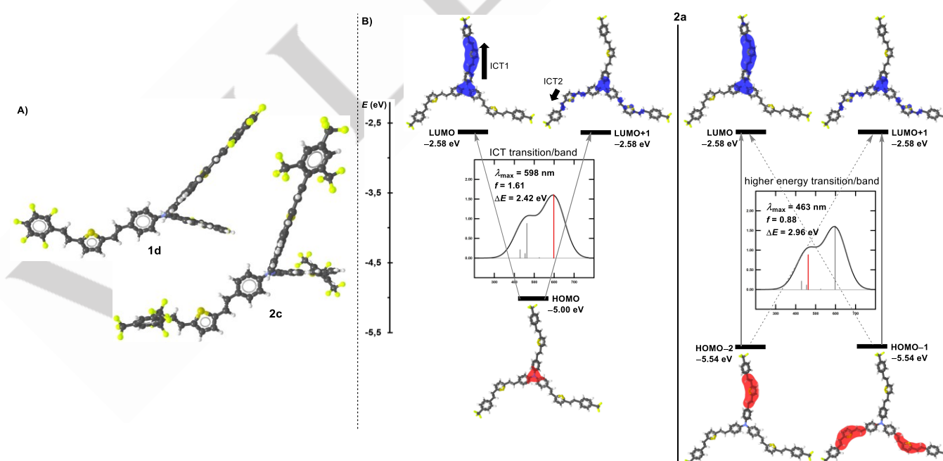
Figure 5. A) Optimized geometries of fluorophores 1d and 2c calculated using DFT B3LYP/6-311+G(2d,p) level; color of atoms: carbon – black, hydrogen – white, nitrogen – blue, sulfur – yellow, fluorine – yellow-green. B) The principal electron transitions, FMOs and DFT-calculated parameters of the representative trifluoromethyl derivative 2a [the HOMO(–1,–2) are shown in red, the LUMO(+1,+2) in blue; the vertical lines in the calculated absorption spectra represent oscillator strengths ( f )].
