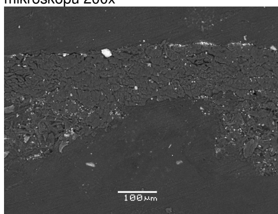
REM-EDS
