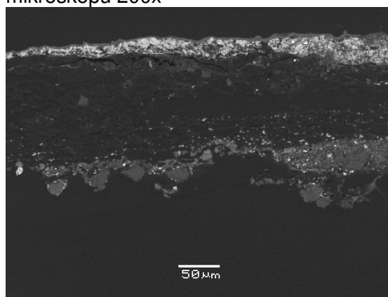
REM-EDS
