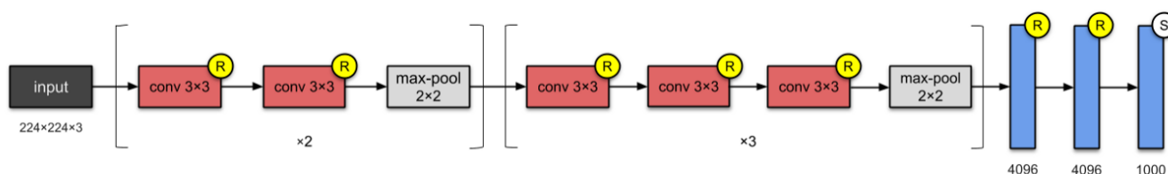
Figure 4. VGG-16 convolutional neural network architecture. Source: (Raimi, 2019).
