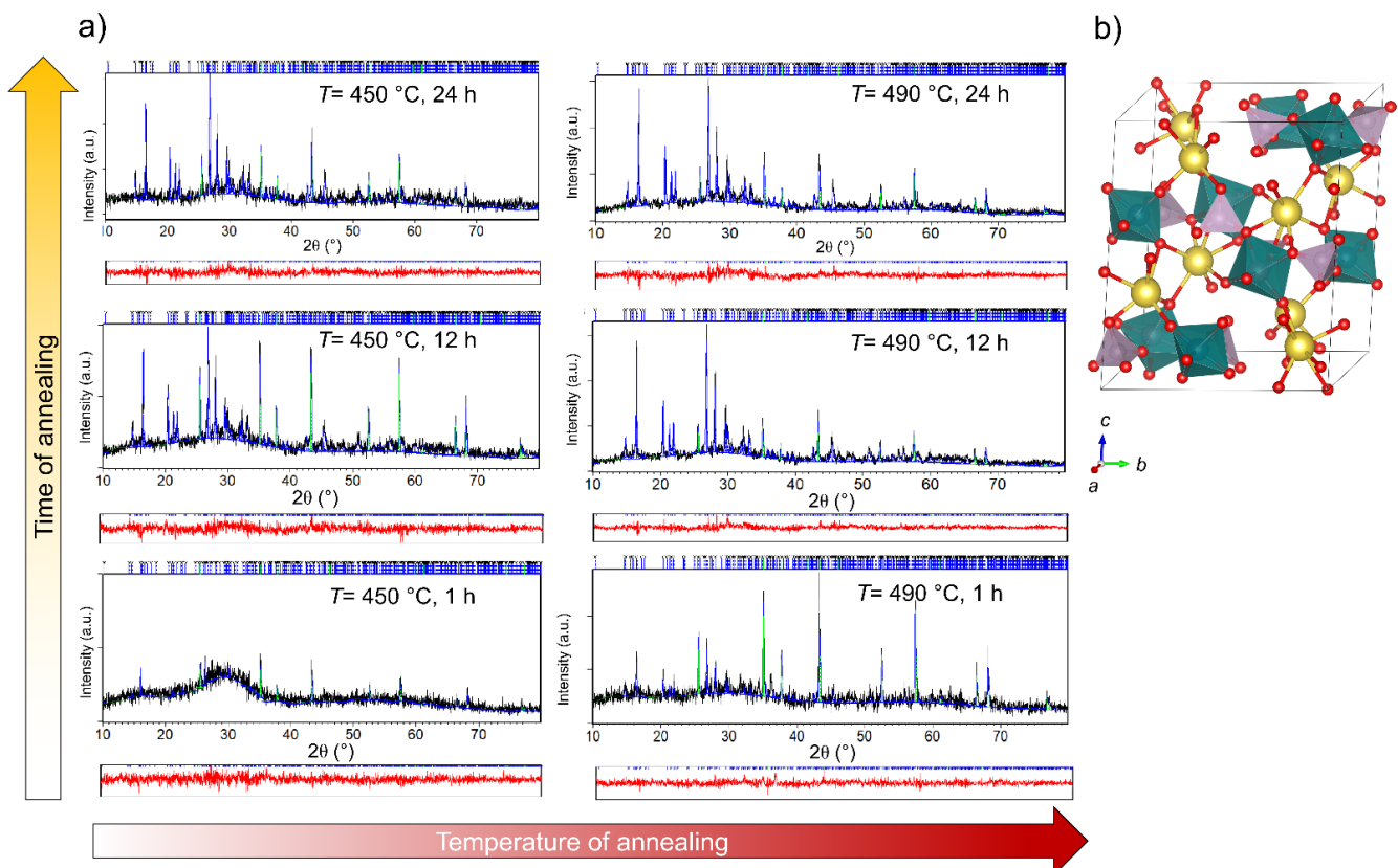
Figure 1. (a) Rietveld refinements of glass samples crystallized at 450 and 490 °C for 1, 12 and 24 h, mixed with powder of \text{Al}_2\text{O}_3 used as an internal standard for amorphous phase quantification. Experimental data are given by the black line, the calculated pattern is shown in blue, and the red line below represents the difference curve. Blue vertical marks show the positions of diffraction lines belonging to \text{NaMoO}_2\text{PO}_4 phase, while the positions of \text{Al}_2\text{O}_3 lines are given as green vertical marks. (b) The structure of \text{NaMoO}_2\text{PO}_4 : Mo is given in teal, P in pink, Na in yellow and O in red.
