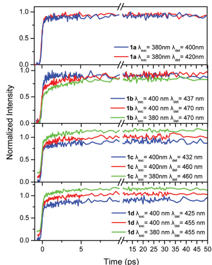
Fig. 4 Fluorescence dynamics within the first 50 ps for the compounds in series 1 in TOL at different excitation/detection wavelengths. An offset is given in some decays for clarity.
