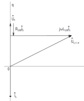
Fig.4 Phasor diagram of the circuit with pulse rectifier and sine filter in the case of mains supply 3x400 V
