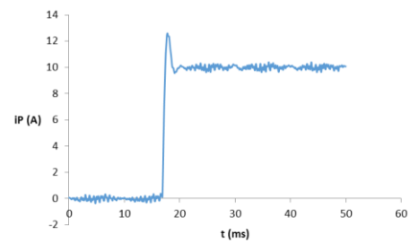
Fig. 6 Response of the current component of the current i_p to the step change of the desired value
