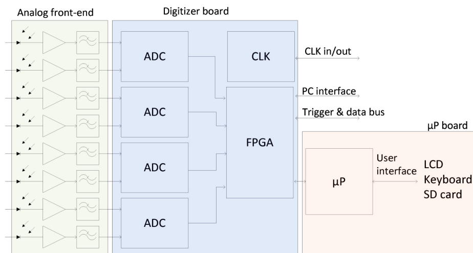
Figure 2. Block schematic of the 8-channel measurement system OPTIMEX
