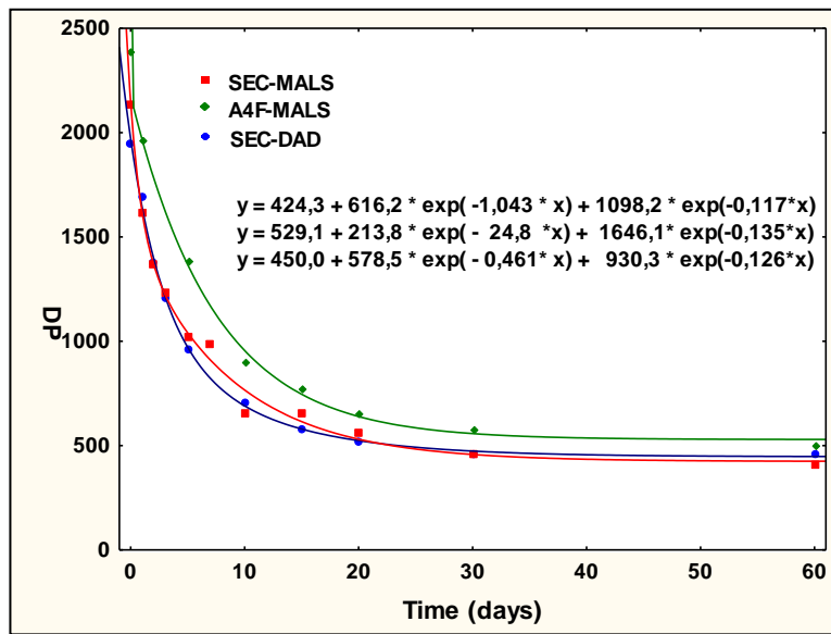
Fig. 1 Degree of polymerization (DP) decrease during accelerated ageing of newspaper paper
