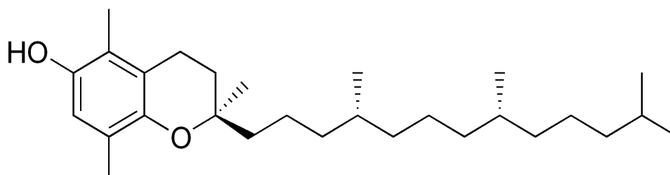
Fig. 1 Chemical structure of \alpha -tocopherol
