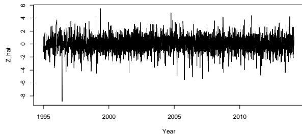
Fig. 6: Volatility-standardised residuals.
