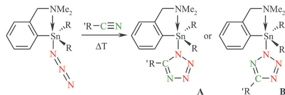
Scheme 2 Preparation of C,N-chelated organotin(IV) tetrazolides 7–14 (for \text{R} = n\text{-Bu} : \text{R} = \text{Me} ( 7 ), t -Bu ( 9 ), \text{Ph} ( 11 ), \text{Me}_2\text{NCH}_2 ( 13 ); for \text{R} = \text{Ph} : \text{R} = \text{Me} ( 8 ), t -Bu ( 10 ), \text{Ph} ( 12 ), \text{Me}_2\text{NCH}_2 ( 14 )). A = C,N-chelated organotin(IV) 5- R -tetrazol-1-ide regioisomer; B = C,N-chelated organotin(IV) 5- R -tetrazol-2-ide regioisomer.
