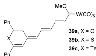
Fig. 26 Chalcogenapyrans in push–pull Fischer type carbene complexes.
