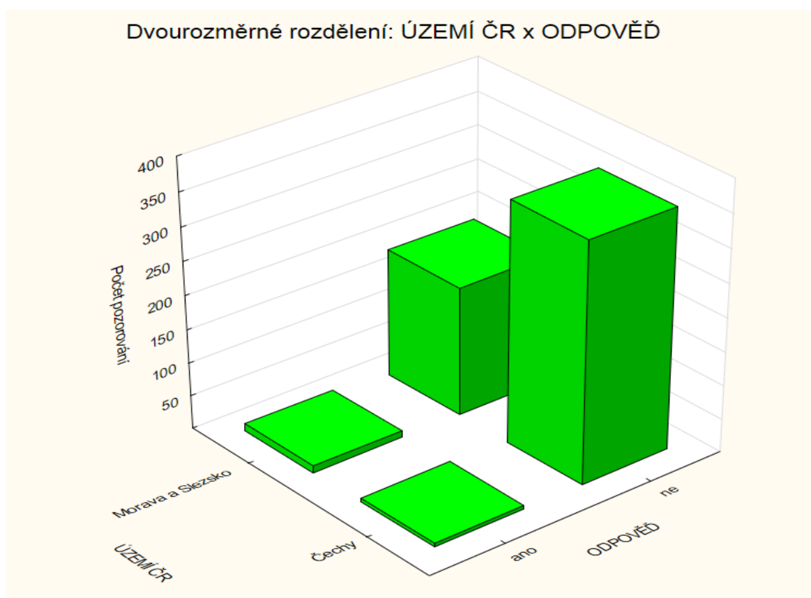
Graf 4 3D histogram
