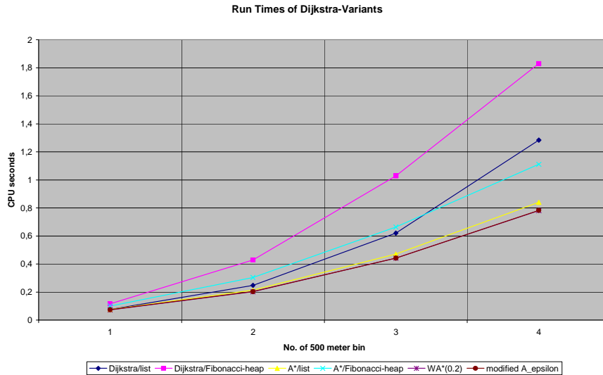
Fig. 3: run times of several Dijkstra-variants for smaller distance
