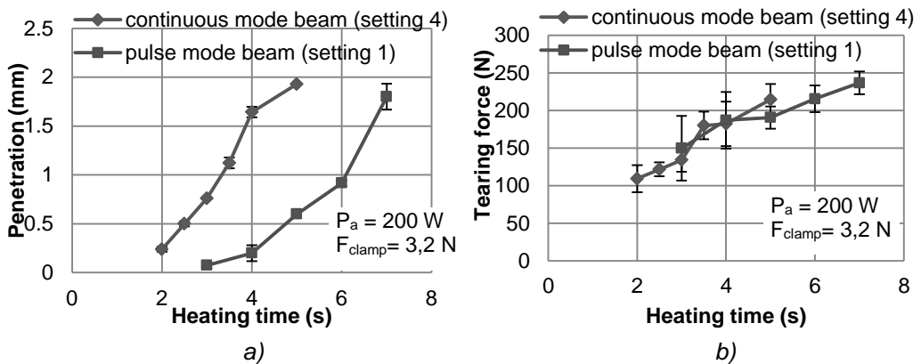
Fig. 2 Penetration (a) and tearing force (b) of joints as a function of heating time in case of pulse mode and continuous mode laser beam joining
